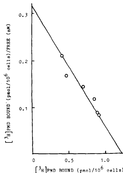
Fig.1. Scatchard plot for the specific binding of [ ^3 H]PMD to cultured HEFs. Cells were grown in a standard serum medium at a density of 5-7 \times 10^3 cells/cm ^2 . 10^6 cells correspond to 0.41 mg protein.
