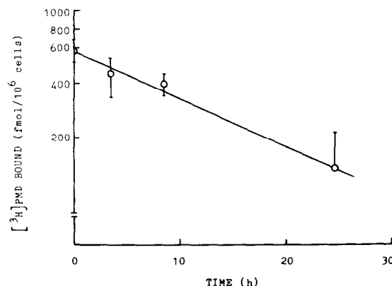
Fig.2. Turnover rate of the DHP receptor in cultured HEFs. Cells were grown at a density of 5-7 \times 10^3 cells/cm ^2 in a standard serum medium containing 10^{-4} M cycloheximide. Changes in [ ^3 H]PMD binding site number were measured at a radioligand concentration of 1.7 nM.
